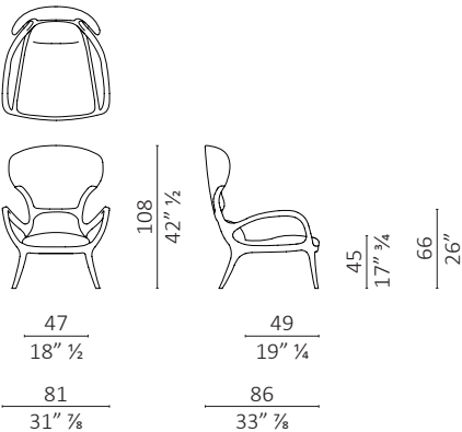
Saturn
