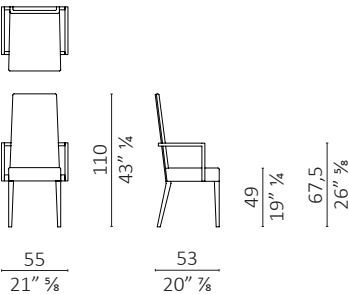
Classic Chair alta con braccioli / high with armrests
