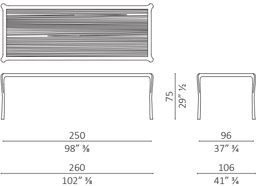
Whity rettangolare / rectangular
