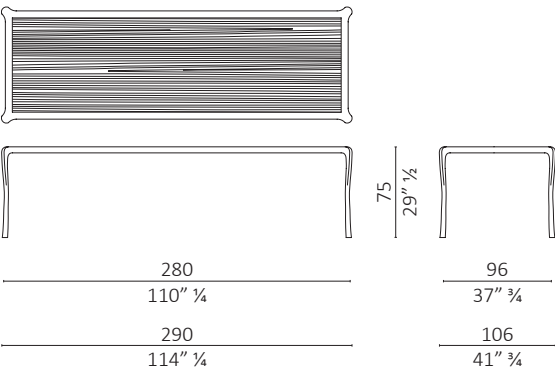
Whity rettangolare / rectangular
