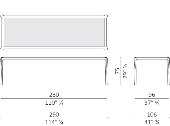
Whity rettangolare / rectangular
