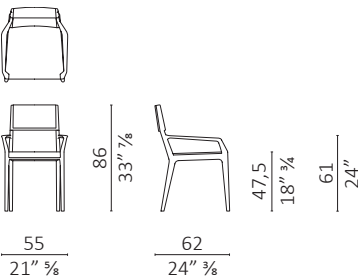
Ala con braccioli / with armrests
